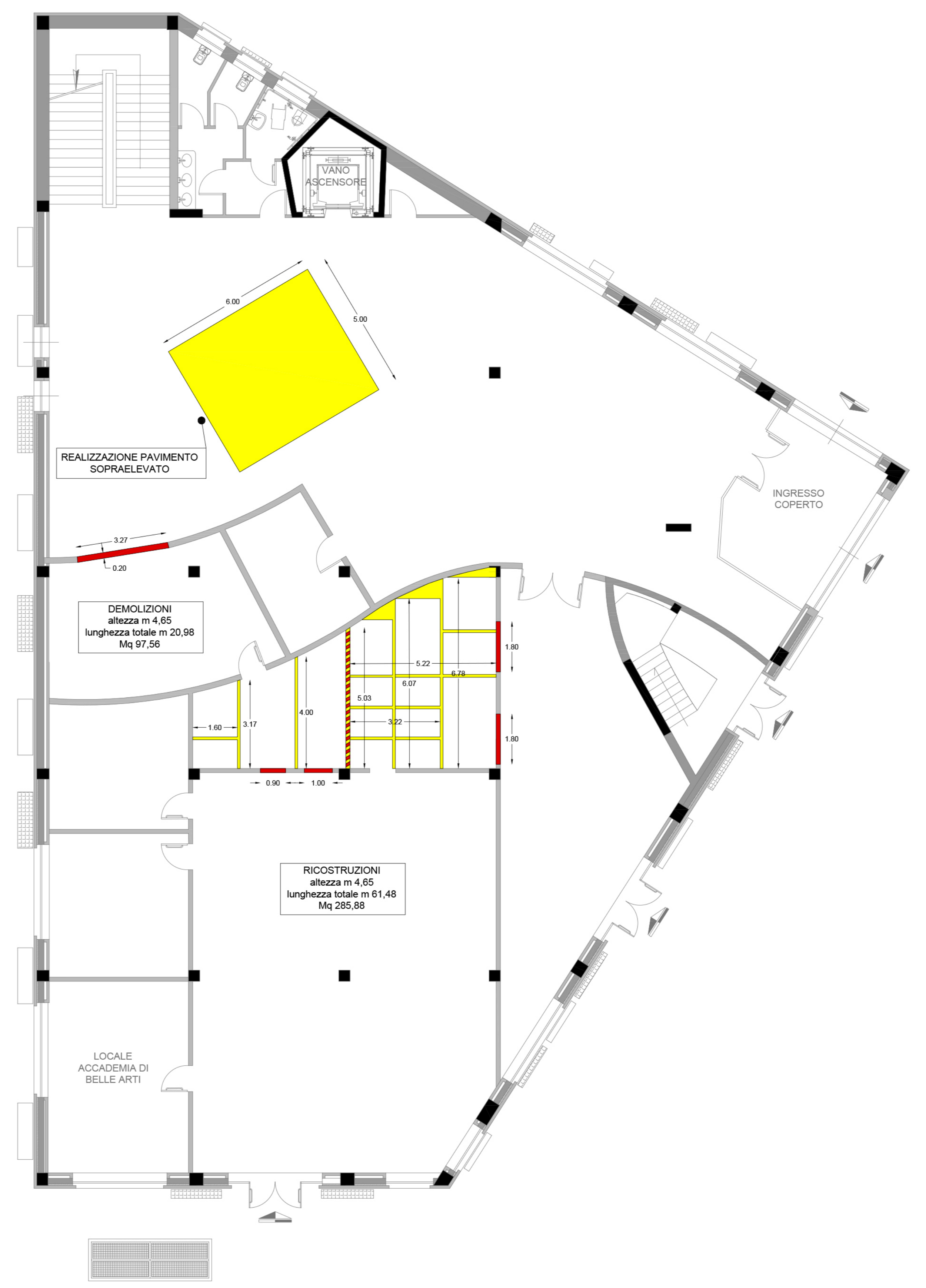
Piano Terra
